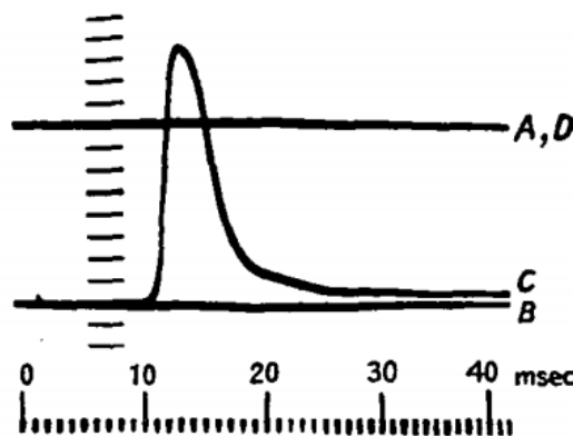
FIG. 1. RESTING POTENTIAL AND ACTION POTENTIAL OF FROG MUSCLE FIBRE
